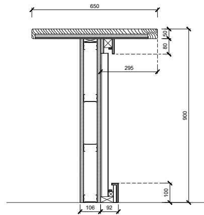
SECTION C SCALE 1:20
