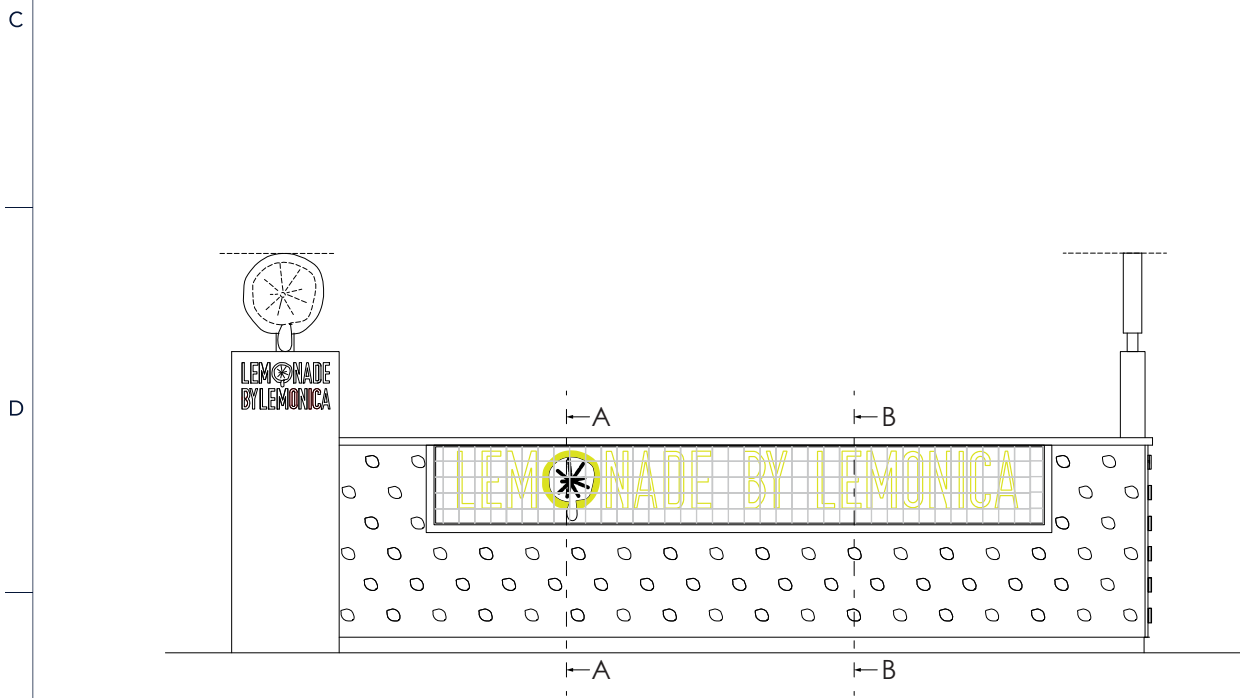
ELEVATION VIEW
