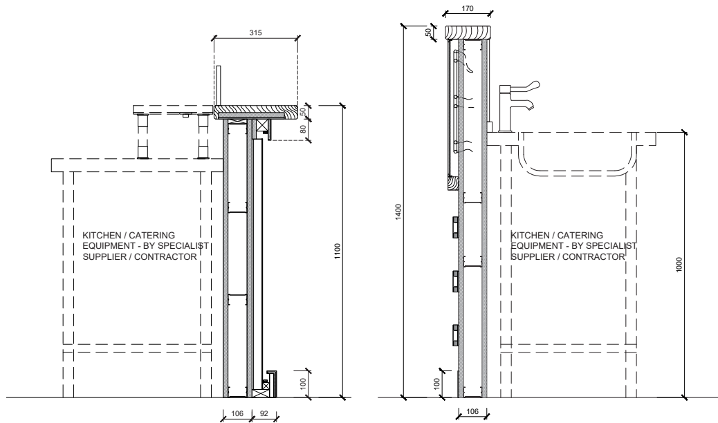
SECTION A SCALE 1:20
