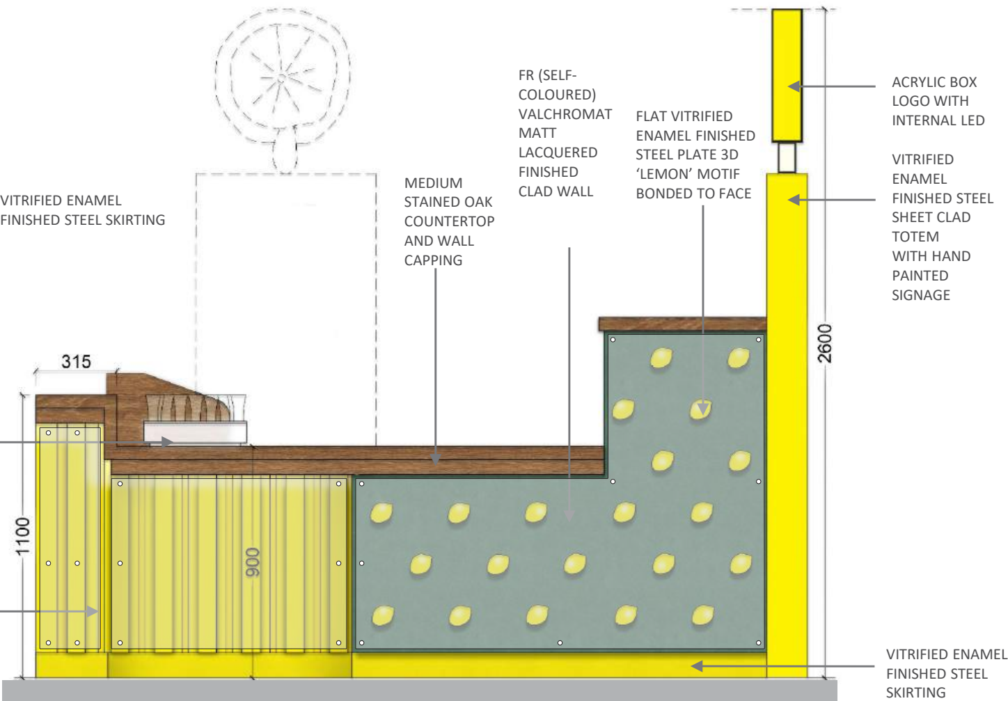
ELEVATION CC
