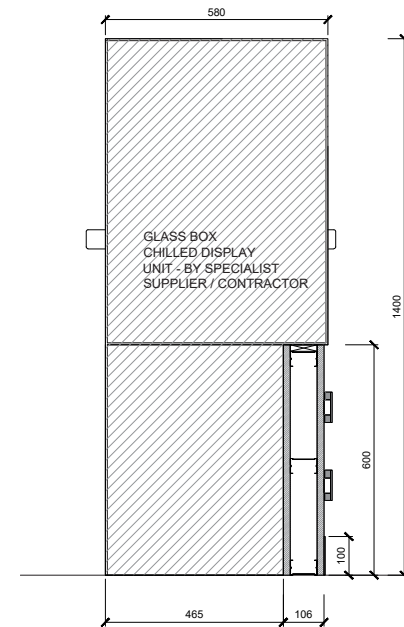
SECTION E SCALE 1:20
