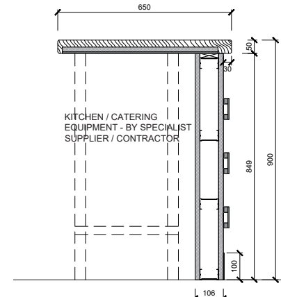
SECTION D SCALE 1:20
